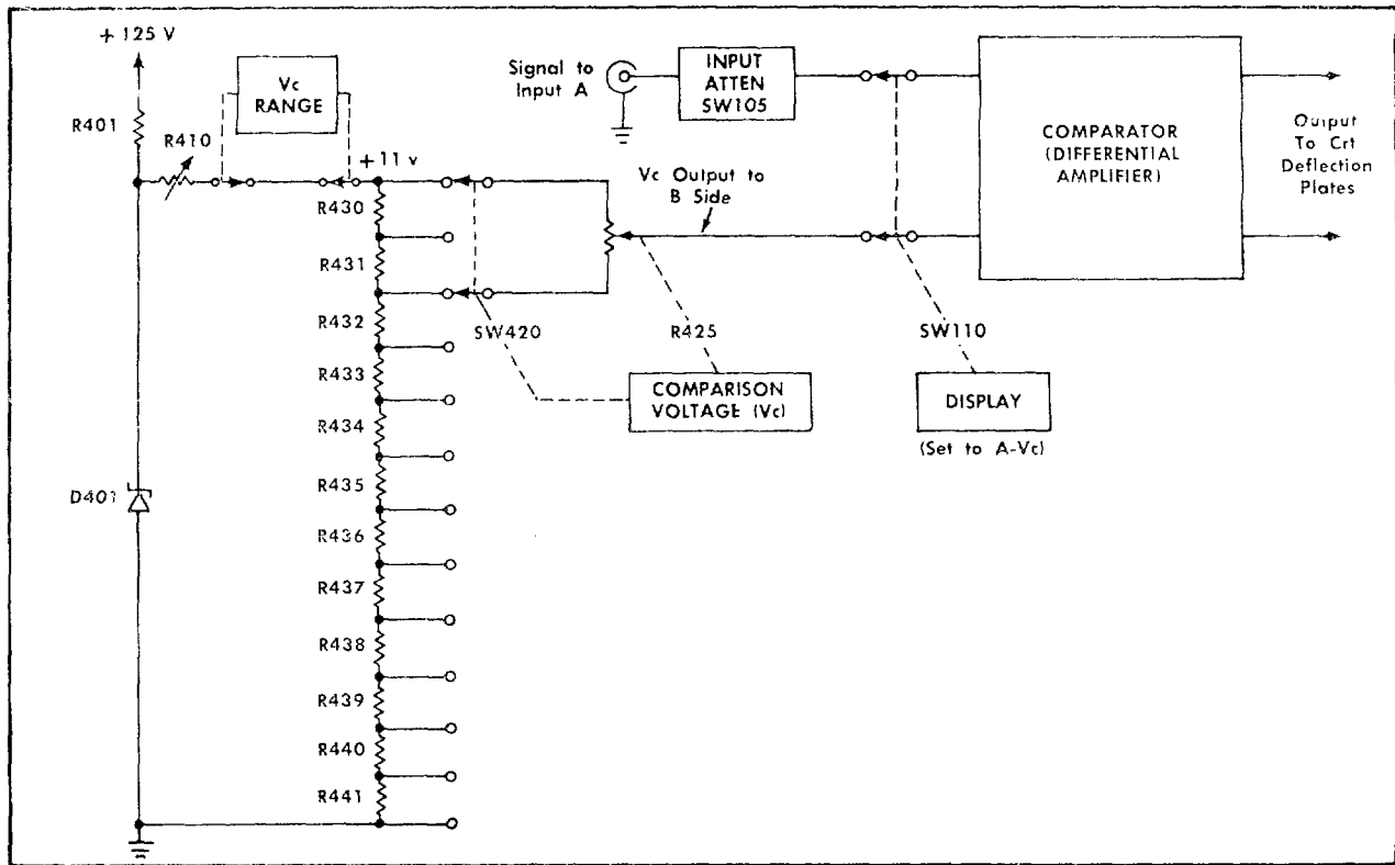
Fig. 3-1. Simplified diagram of the comparison voltage circuit and how it is connected to the amplifier for A-Vc differential-comparator mode of operation.
